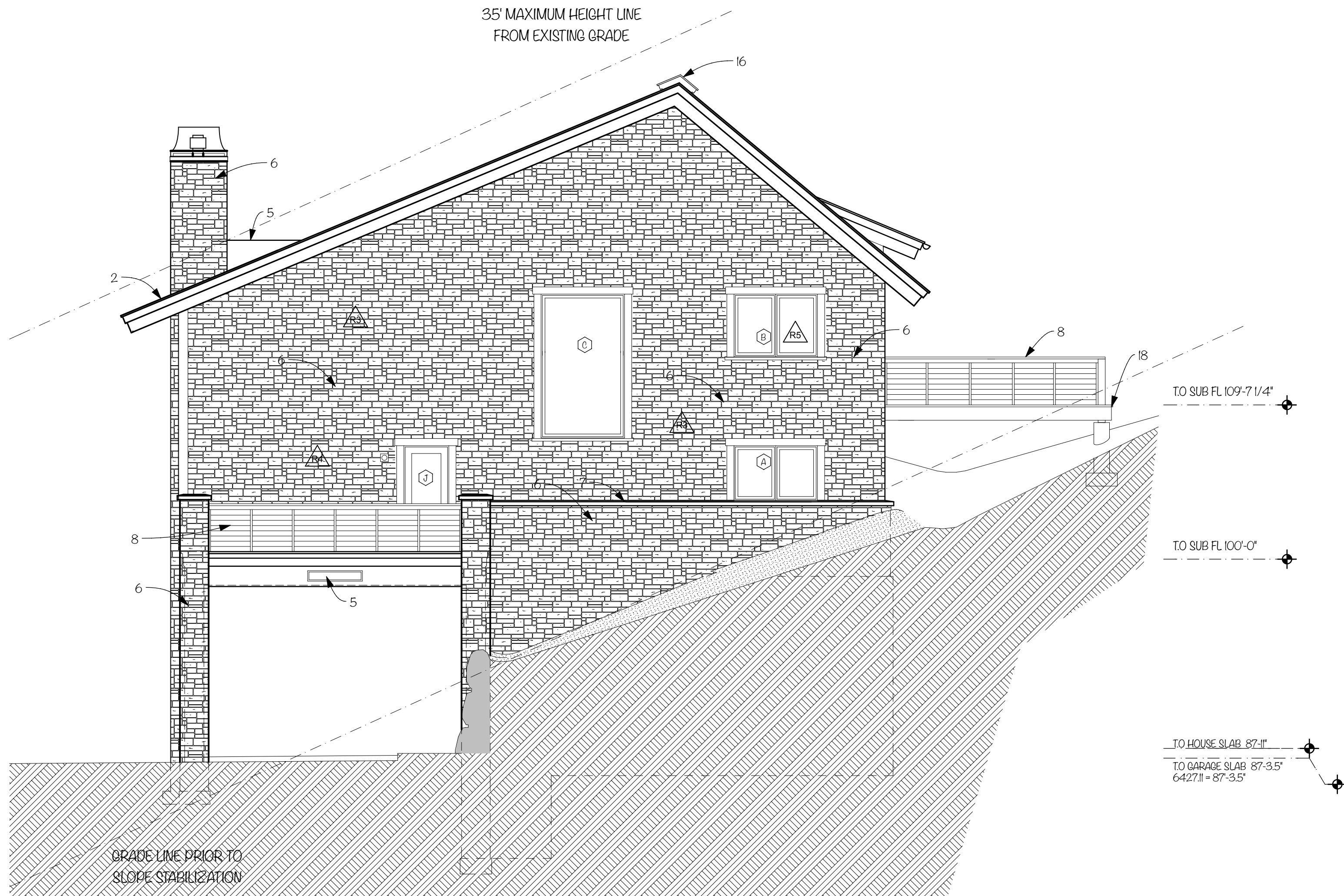
WEST ELEVATION
