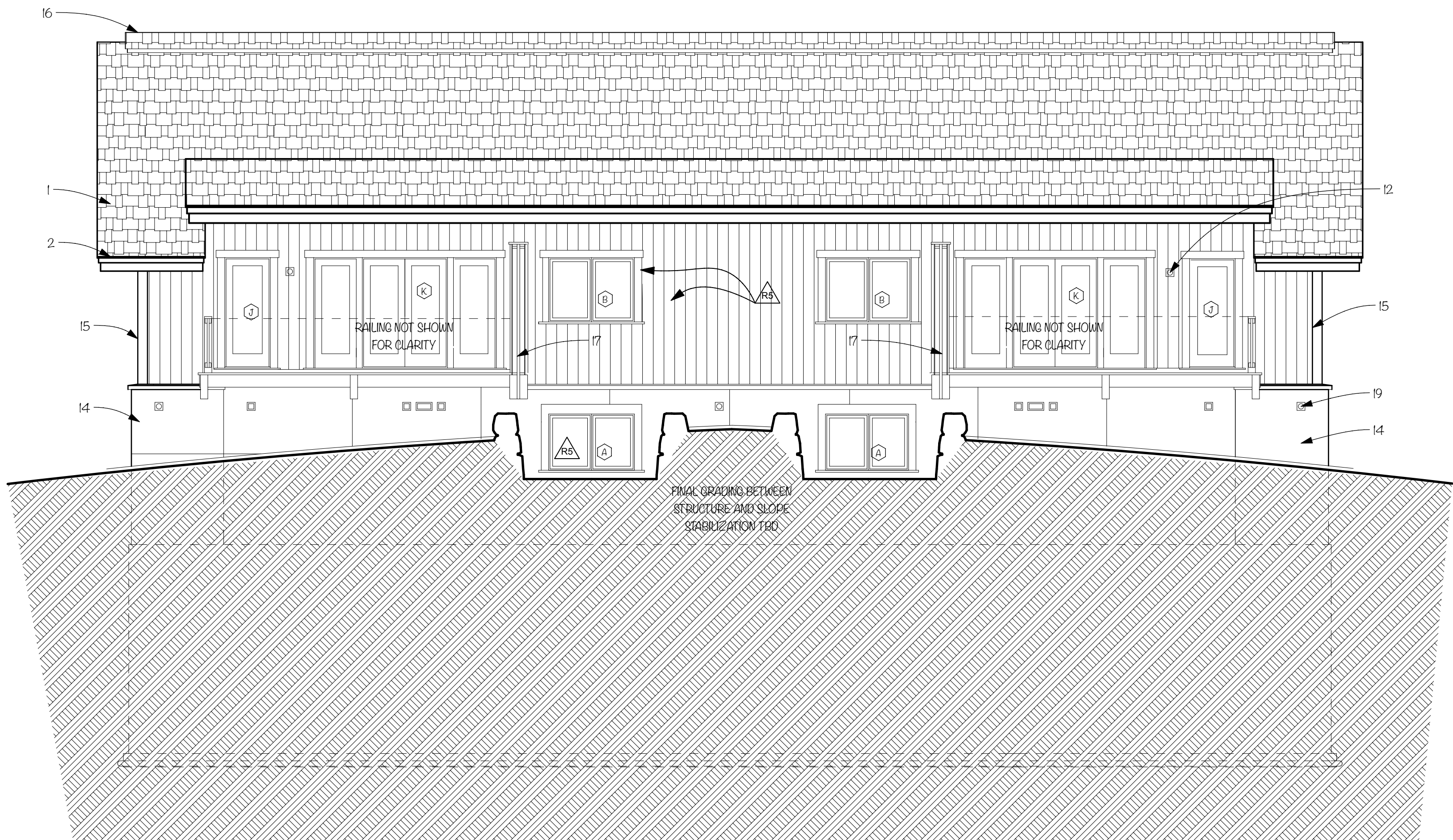
SOUTH ELEVATION
