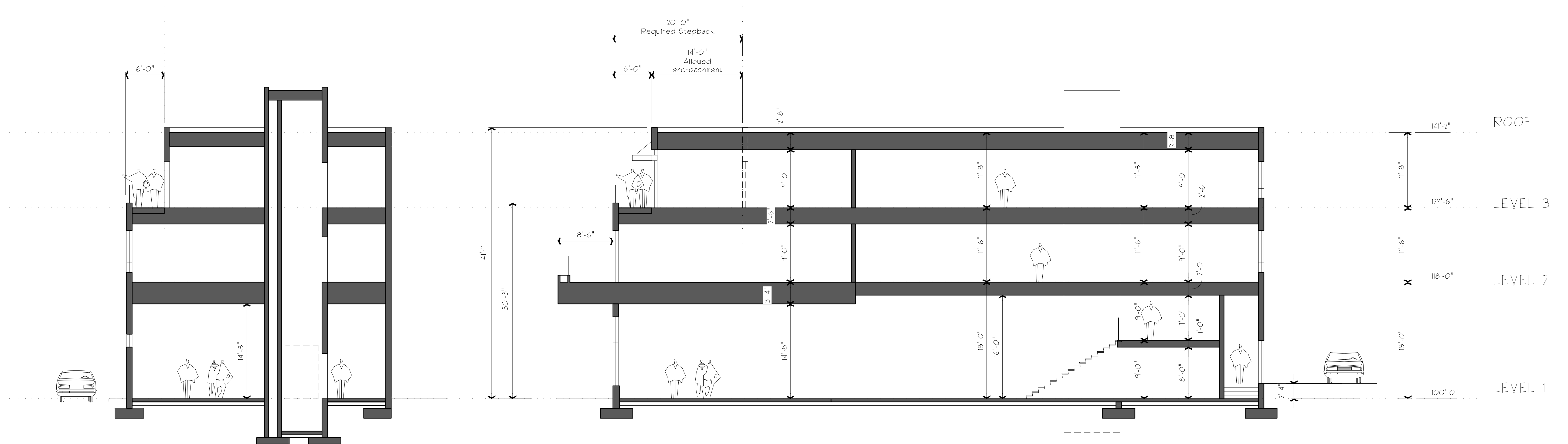
BUILDING SECTION A-A
