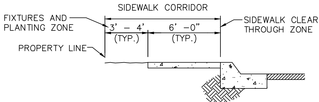
ATTACHED SIDEWALK (NON-COMMERCIAL STREETS) (SEE NOTE 4)
