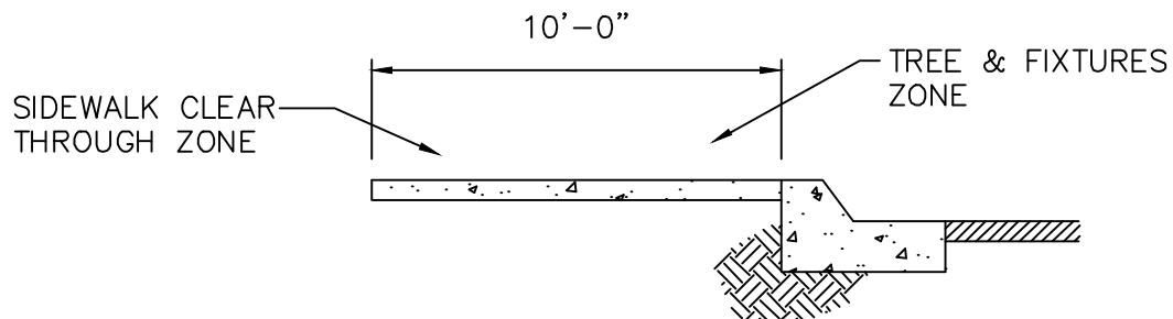
ATTACHED SIDEWALK (COMMERCIAL STREETS)
