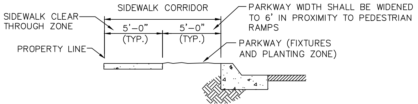
DETACHED SIDEWALK (SEE NOTE 5)
