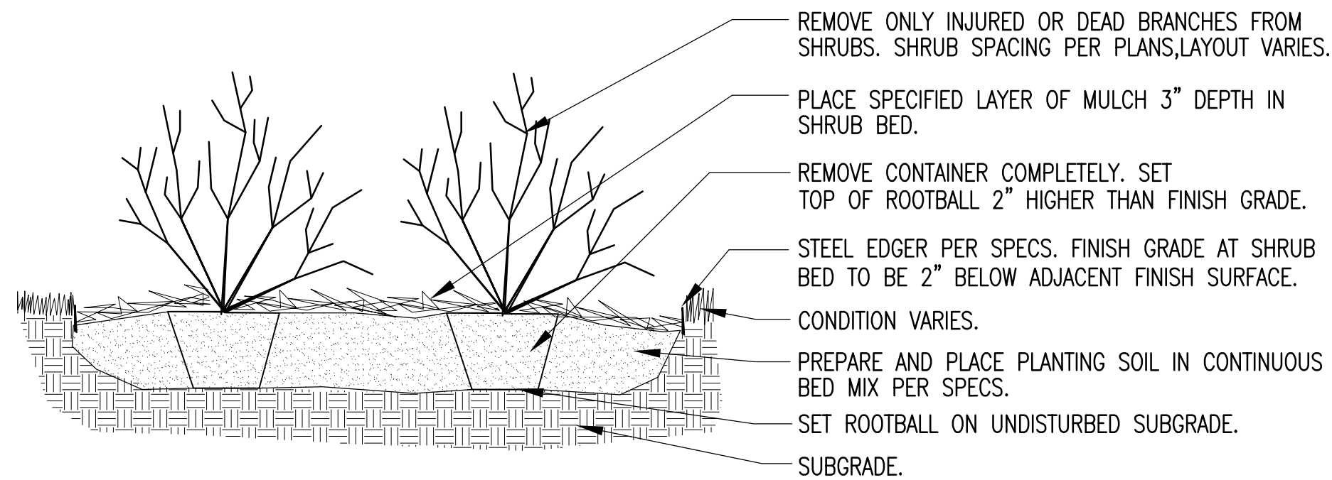
4 PERENNIAL PLANTING NTS
