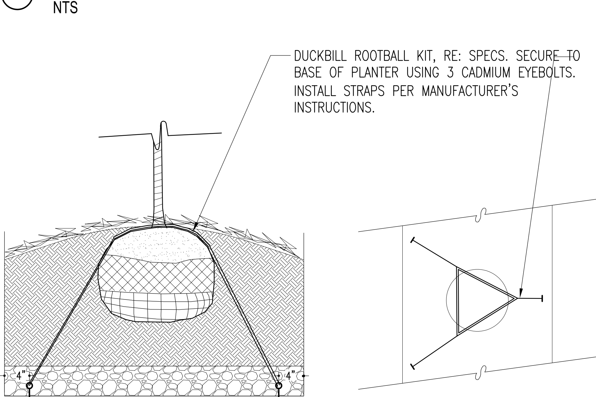
6 PLANTER TREE STRAP NTS
