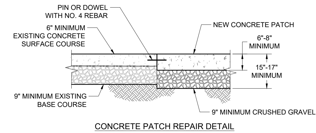
CONCRETE PATCH REPAIR DETAIL
