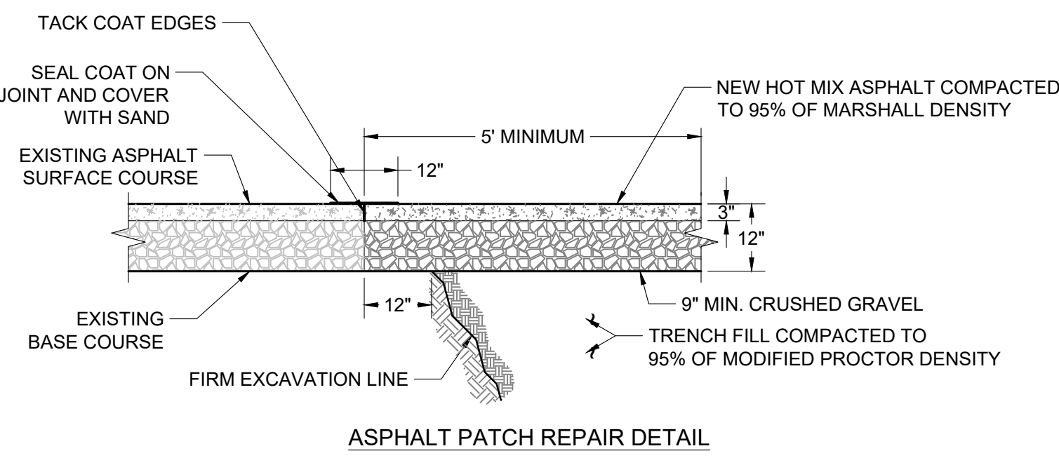
ASPHALT PATCH REPAIR DETAIL
