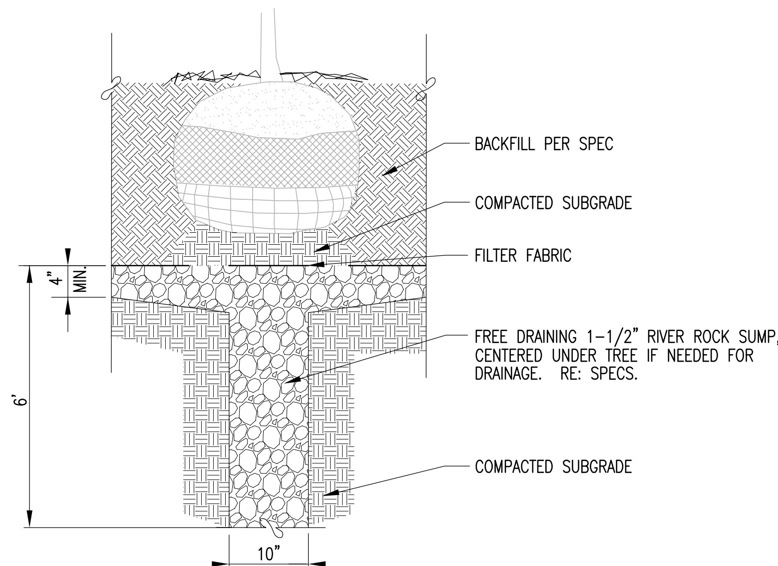
5 TREE PIT DRAIN NTS
